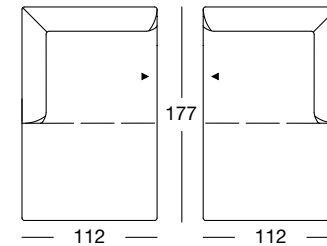
K-UE-ASS-PSZ 160/112 li
